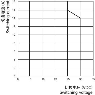
允许最大负载范围 (23°C) Max.imum allowable load range
