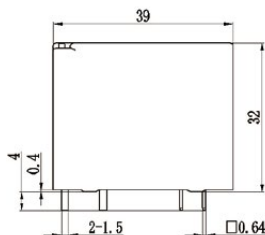
单线圈 Single Coil
