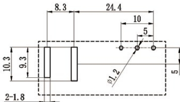
双线圈 Double Coils
