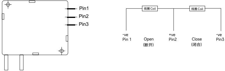
双线圈 Dual Coils
